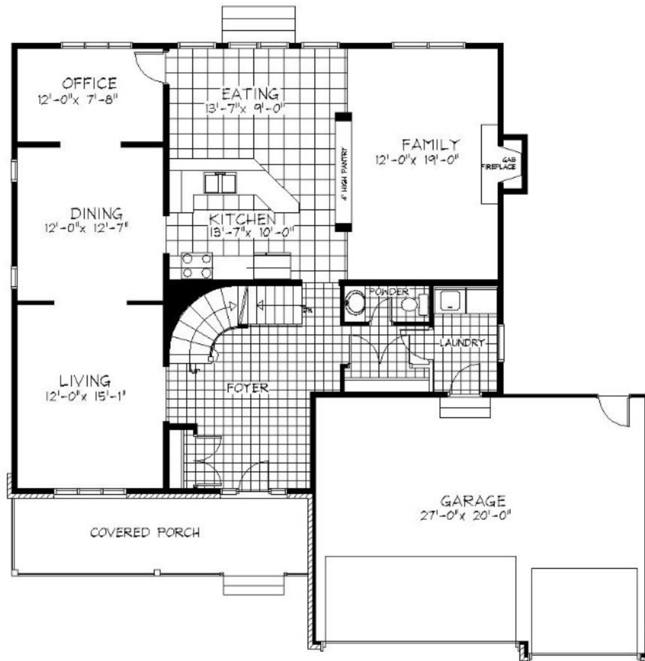
Ground Floor
